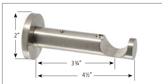
Single Steel Bracket DSS41/SST
