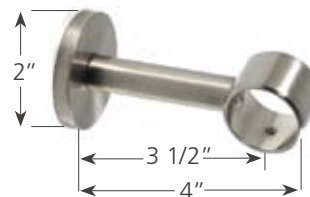
WALL/CEILING BRACKET DTX44/STL
