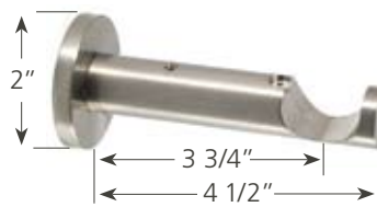
SINGLE STEEL BRACKET DTX41/STL
