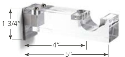
SINGLE CLEAR ACRYLIC BRACKET DTX45/ACR
